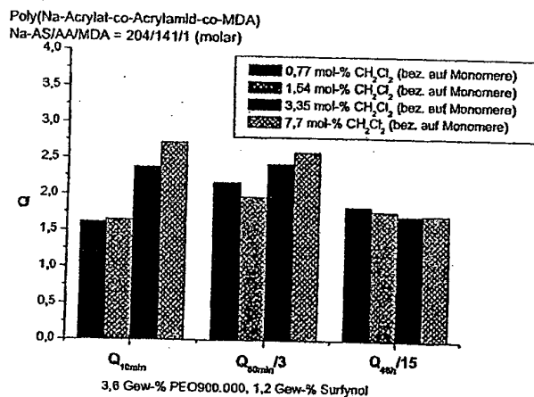
Fig. 11: Swelling experiments of acrylamide/sodium acrylate/MDA hydrogels using PEO 900,000 as rheological additive - Effect of CH 2 Cl 2 as foaming agent
